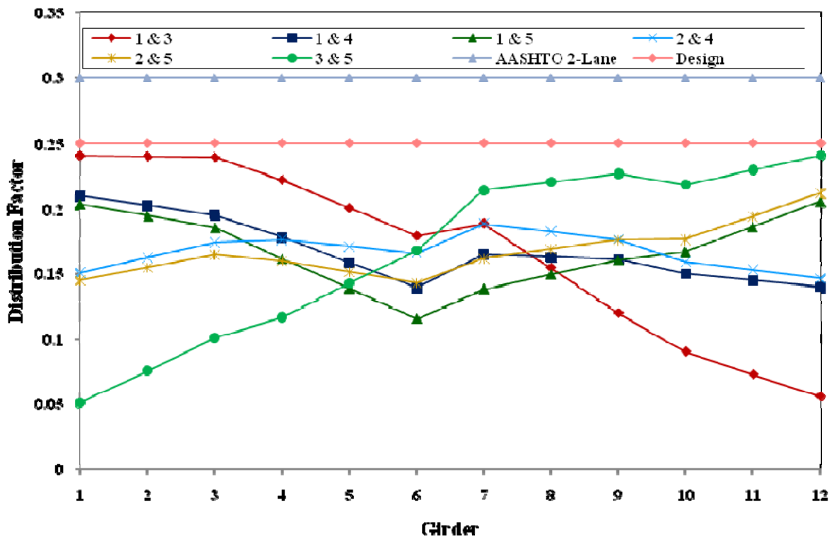
Figure 5.10. Two lane DF from deflections
