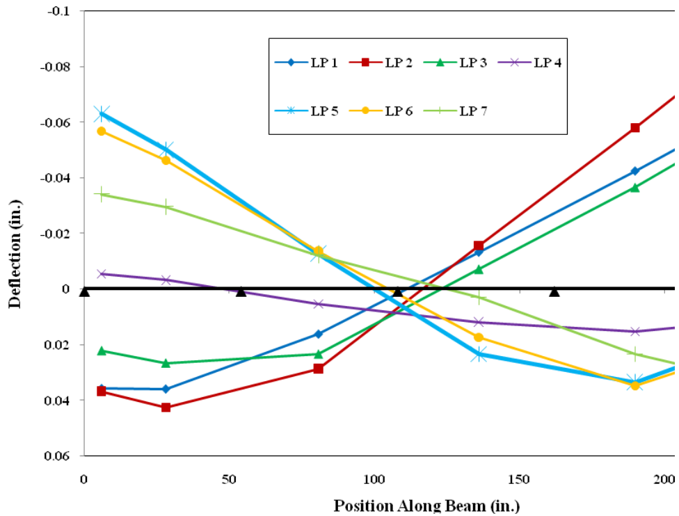
Figure 3.5. Deflection profile for Cap 1 for the seven load points used
