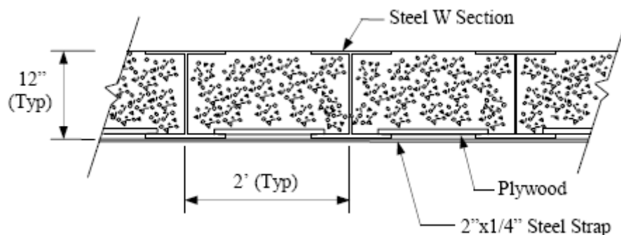
Figure 1.1. BISB cross section
