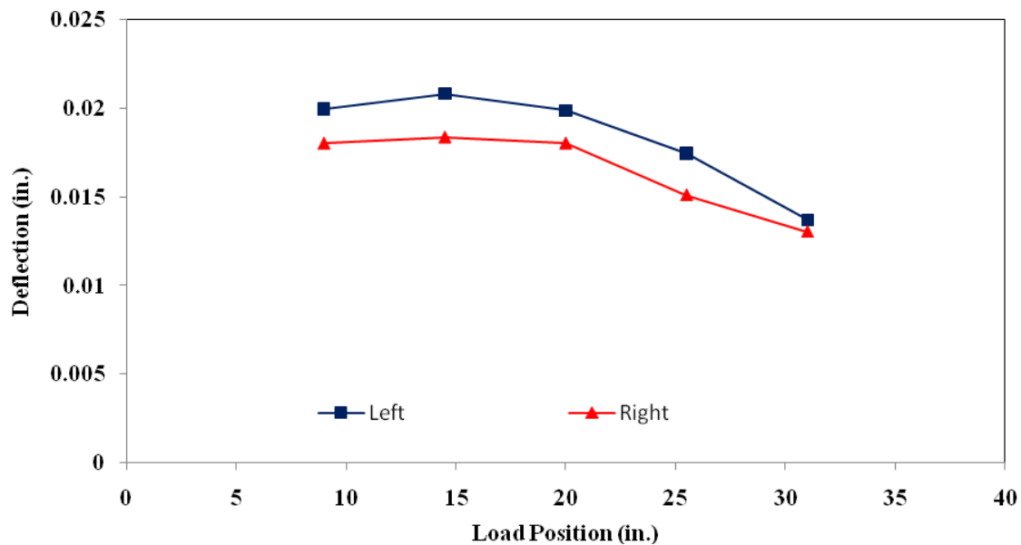
Figure 3.15. Type 2 Connection service deflections
