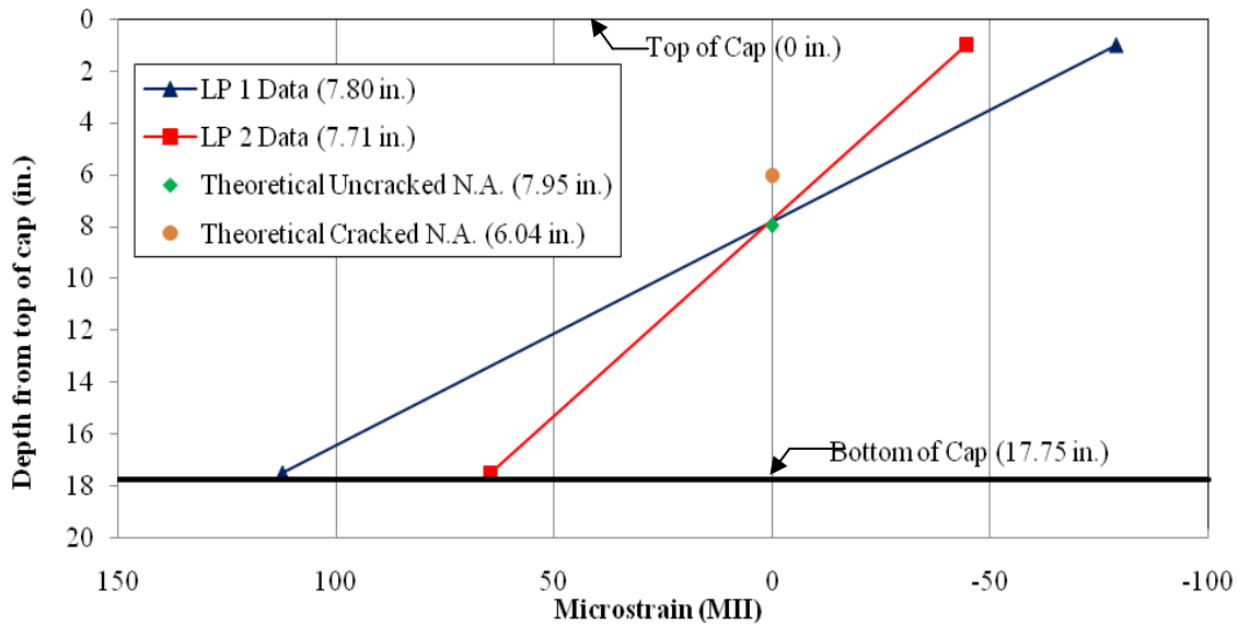
Figure 3.11. Cap 2 neutral axis at Section 1, Load Positions 1 and 2, at 40 kips
