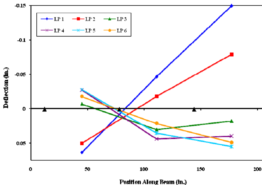
Figure 3.6. Deflection profile for Cap 2 for the six load points used
