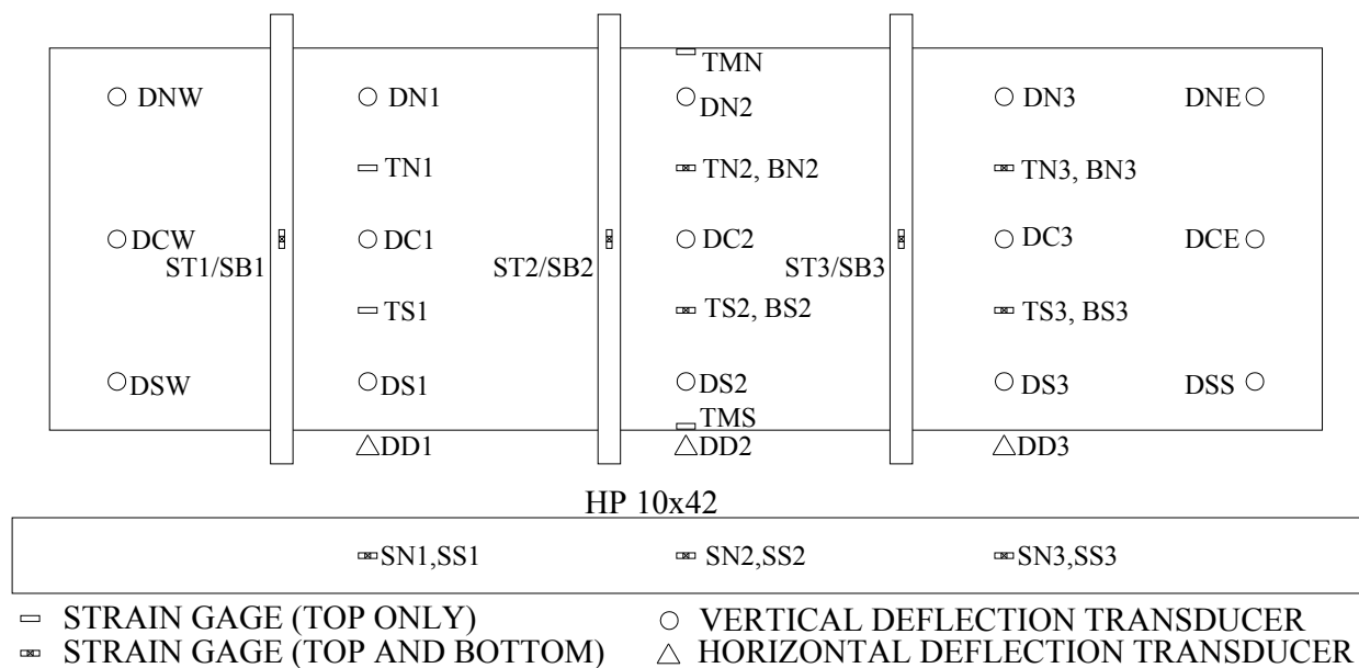
Figure 3.18. Labels for the abutment backwall instrumentation
