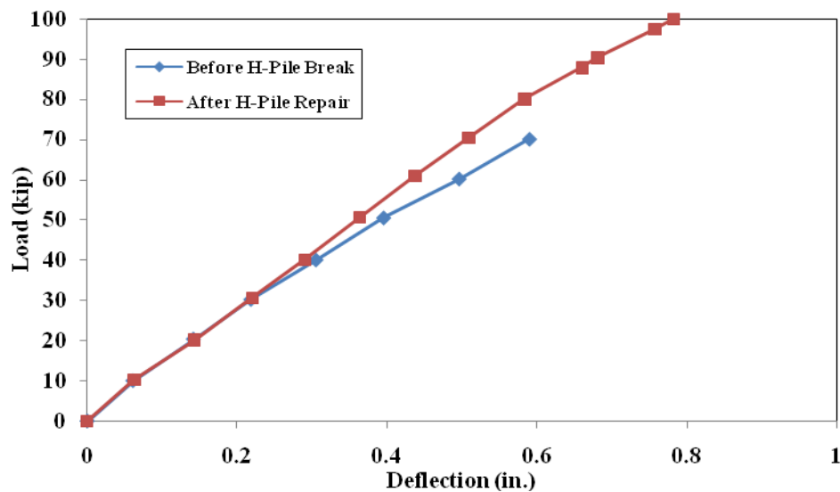
Figure 3.21. Load-deflection curves for strength testing at DC2 before and after HP break
