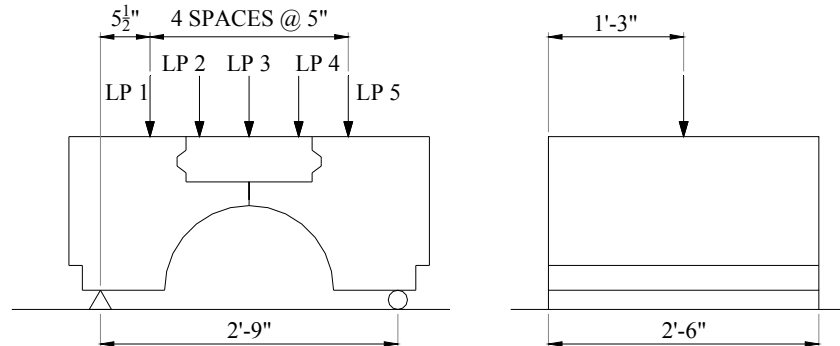
a) Side and end views of service load points
