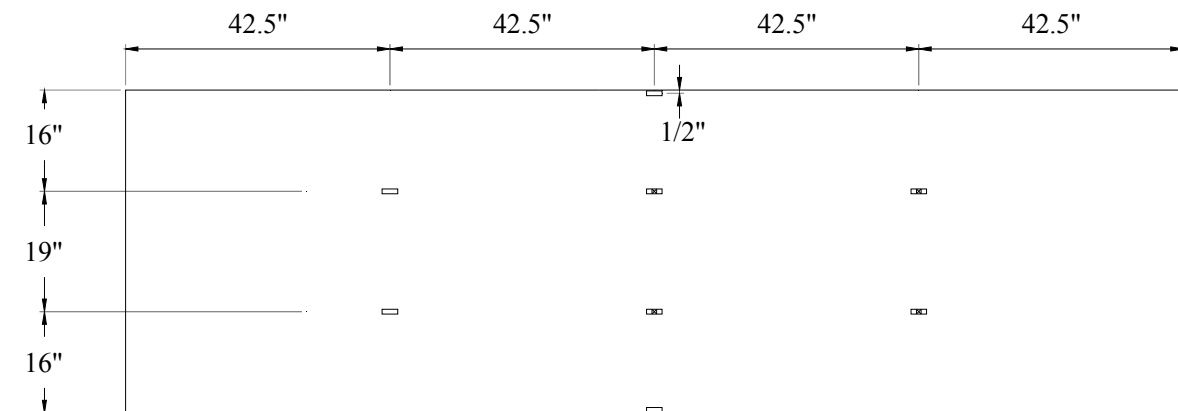
a) Abutment backwall
