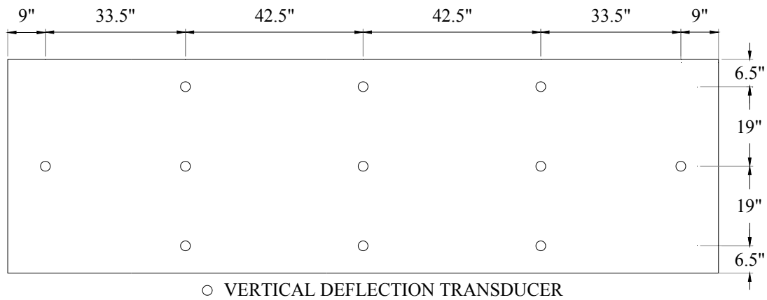
Figure 2.36. Location of deflection transducers for abutment backwall service load test
