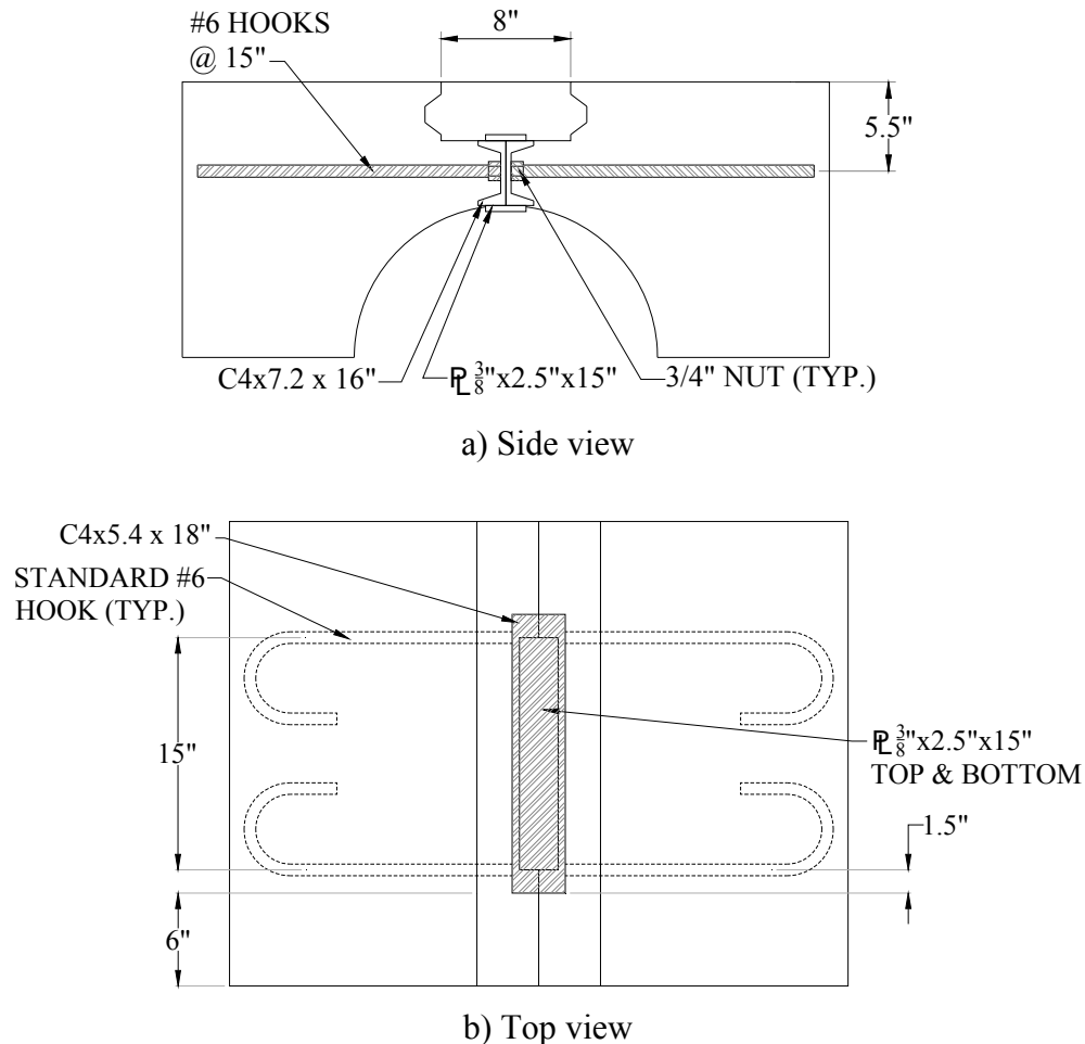
Figure 2.17. Type 2 Connection
