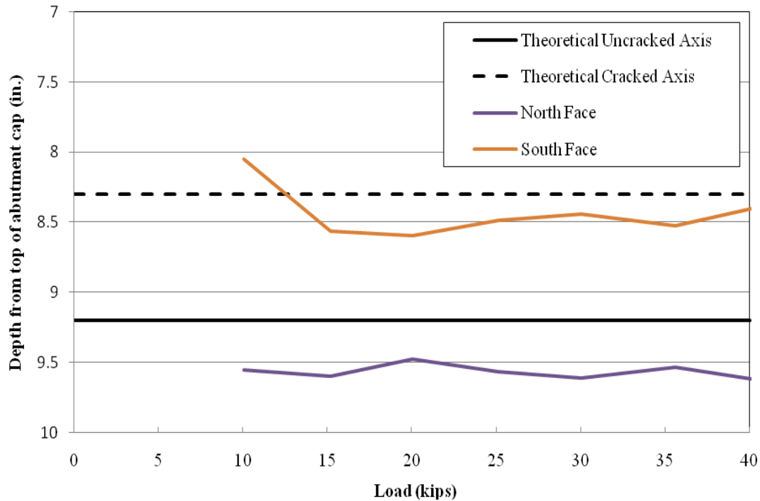
Figure 3.10. Cap 1 neutral axis at Section 2 plotted against load
