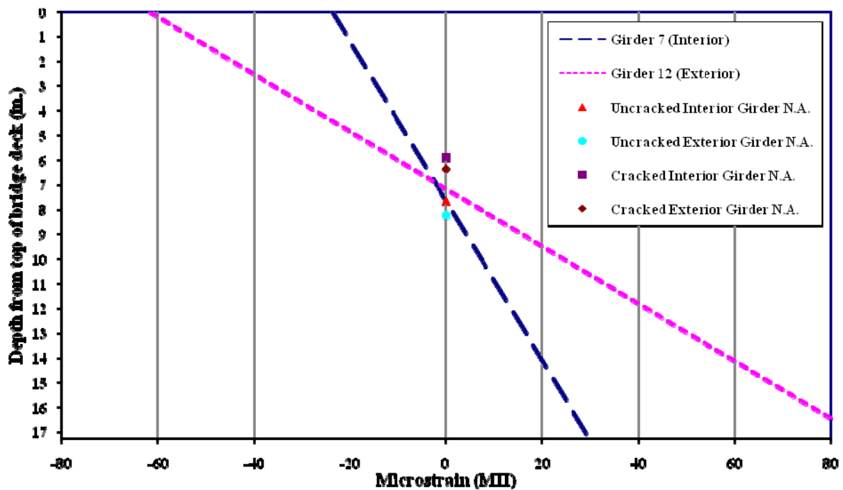
Figure 5.4. Test 5.1 neutral axes
