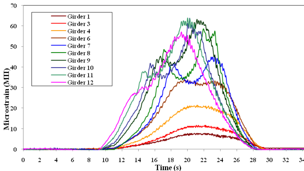
Figure 5.1. Midspan strain history for Test 4.1
