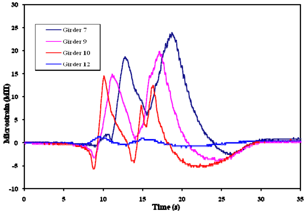
b) East abutment strains
