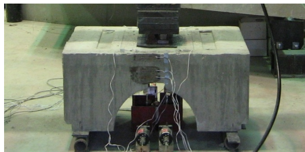
b) Photograph of service test at LP 3
