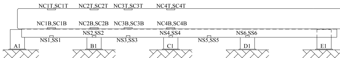
Figure 3.1. Identification of strain gages used on Cap 1
