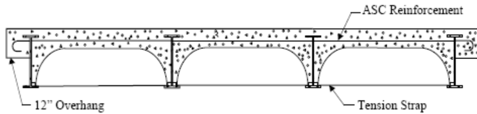
Figure 1.2. MBISB variation 1 cross section
