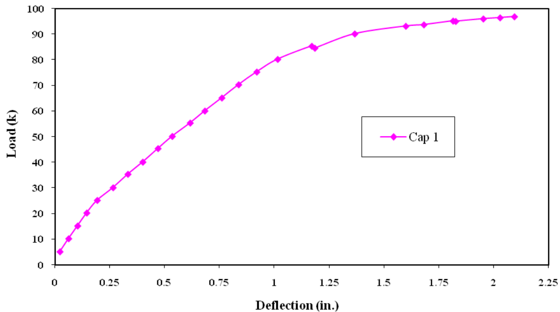
Figure 3.13. Plot of load vs. deflection for negative capacity test of Cap 1
