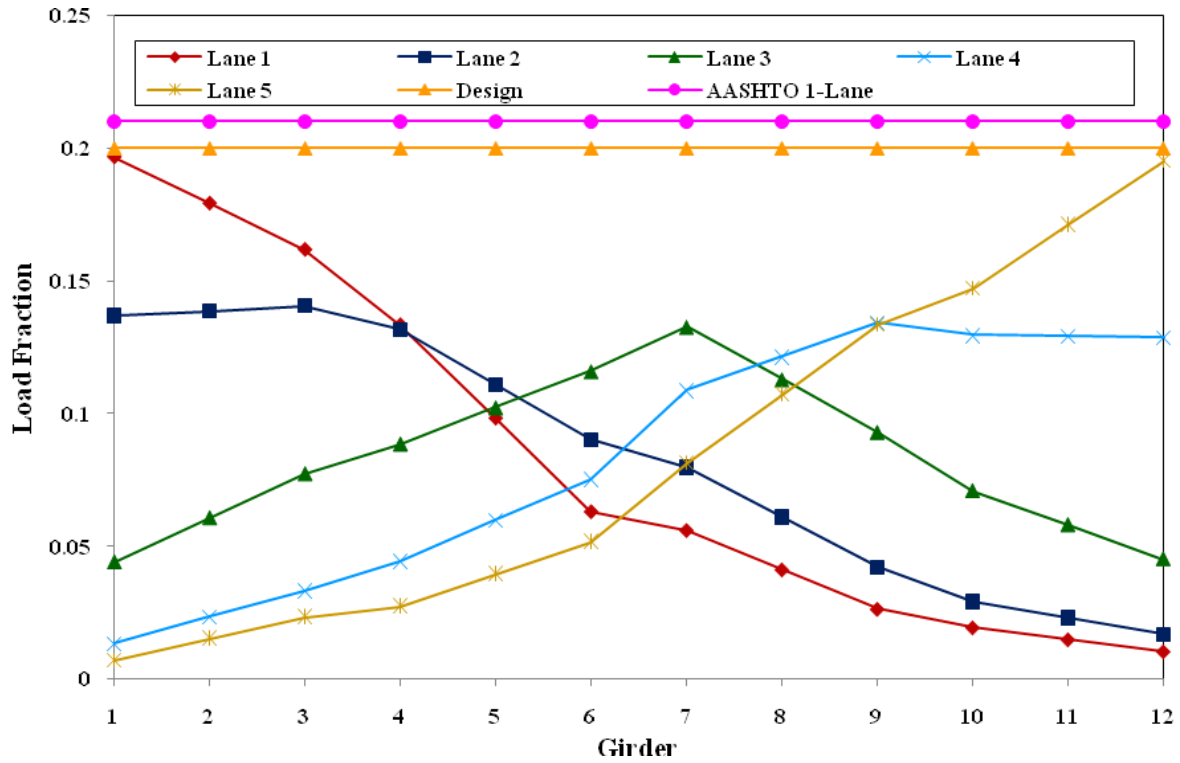
Figure 5.9. Single lane DF from deflections
