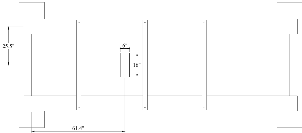
a) Location of load for strength test
