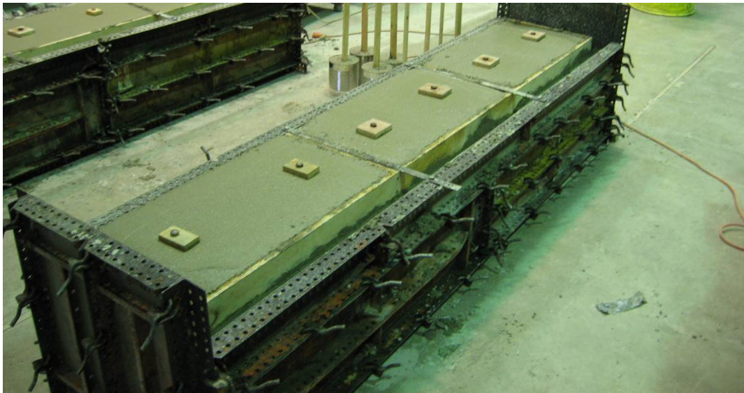
Figure 2.20. Finished concrete and positioned anchors for Type 2 Connection
