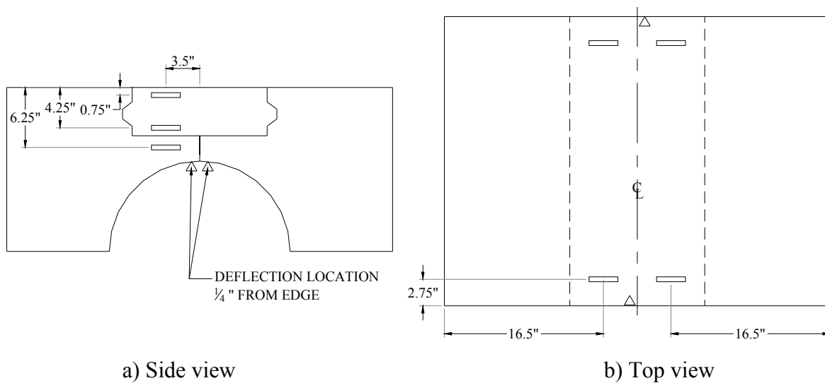
Figure 2.28. Strain gage locations in all three connections
