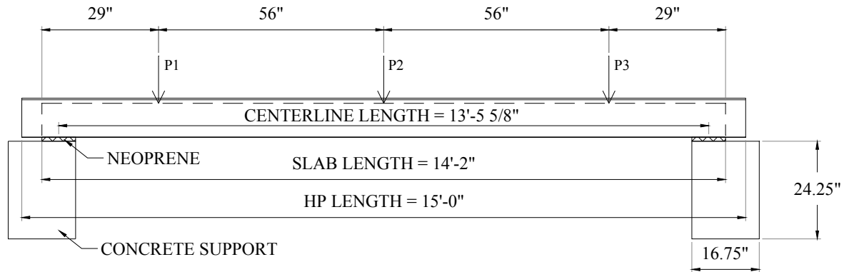
Figure 2.38. Position of loads used in backwall service load tests
