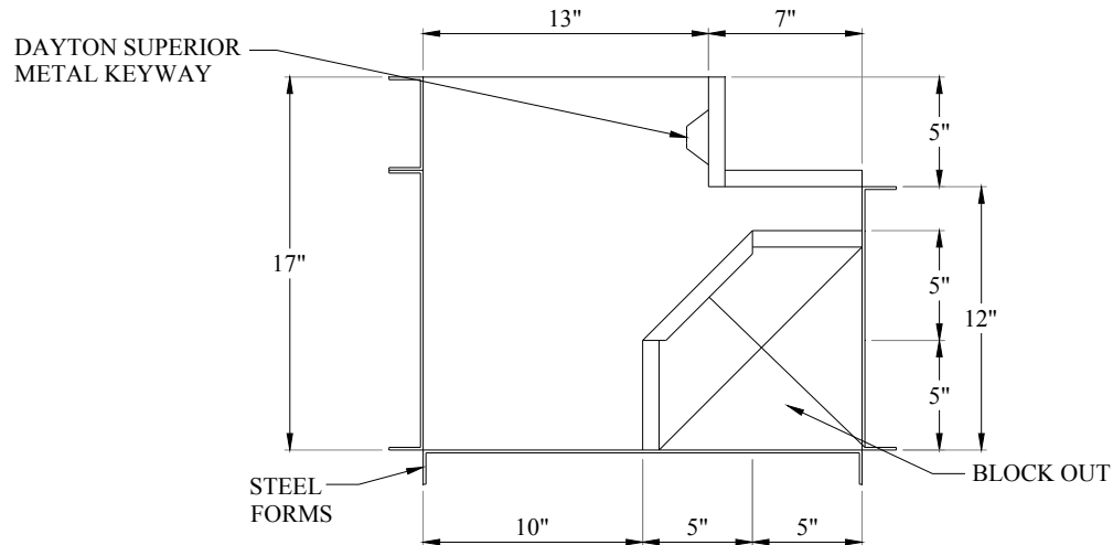
Figure 2.13. Type 1 Connection form details
