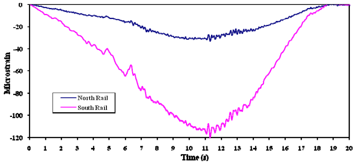
Figure 5.12. Test 3.1 guardrail strains
