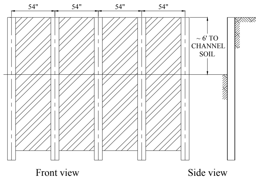
Figure 2.33. Abutment backwalls in the field
