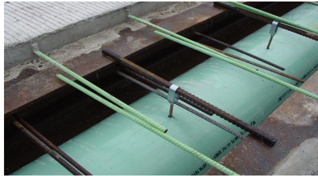
b) Original PMBISB connection in the field
