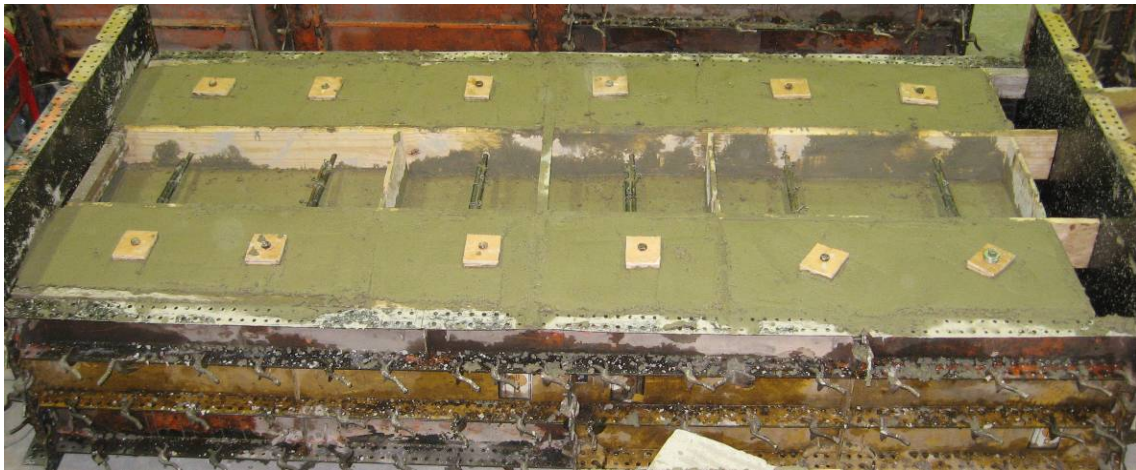
Figure 2.24. Finished concrete for Type 3 Connection
