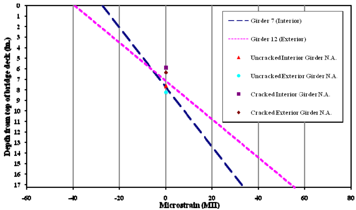
Figure 5.3. Test 4.1 neutral axes
