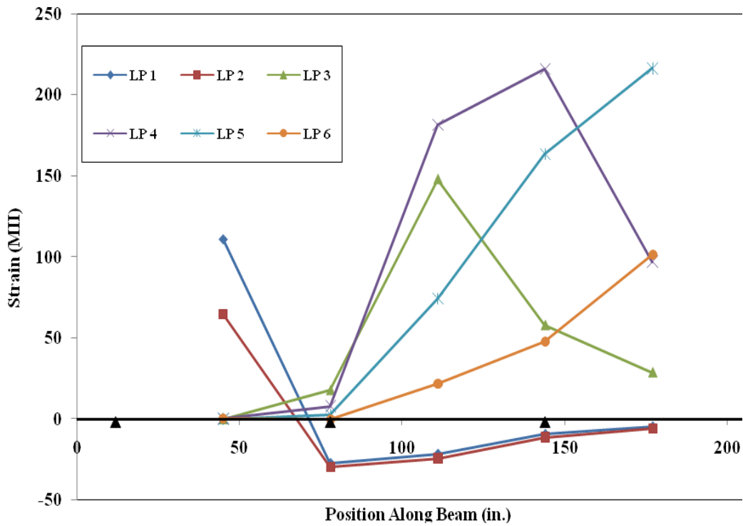
Figure 3.8. Steel strains for Cap 2 for the six load points used
