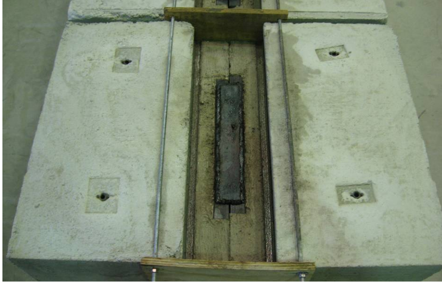
Figure 2.21. Type 2 Connection prepared for closure pour
