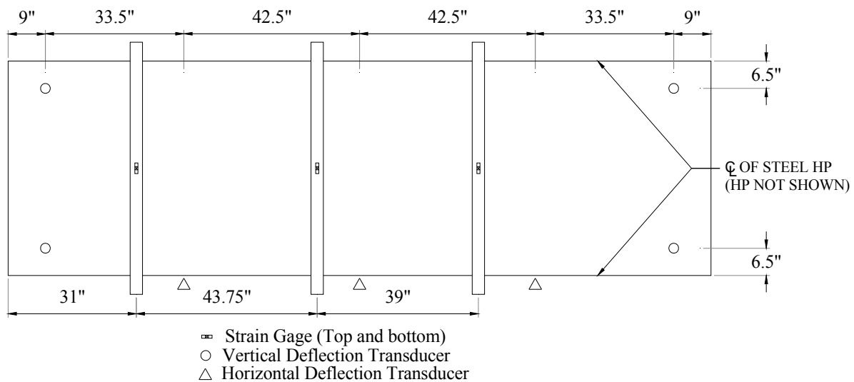
Figure 2.39. Additional instrumentation used in the ultimate strength test of the abutment backwall
