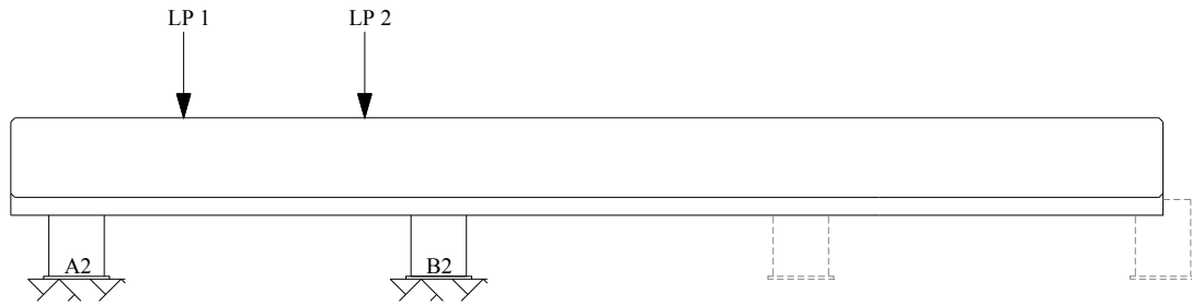
a) Load at LP1 and LP2
