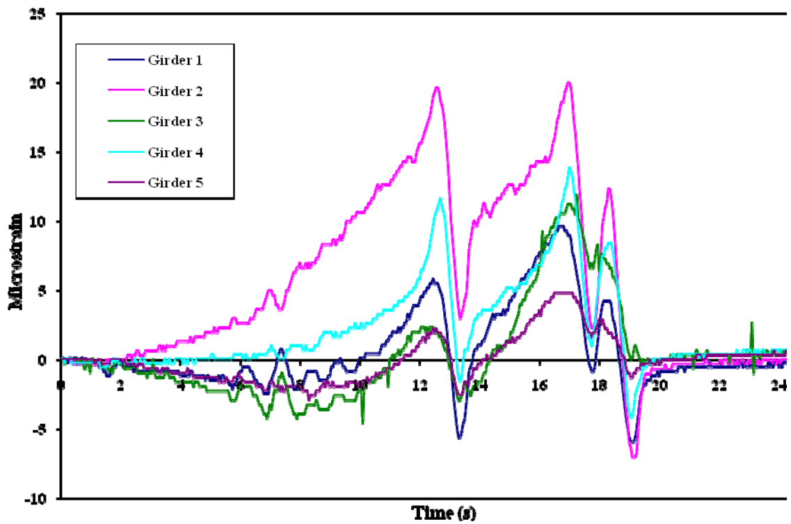
b) West abutment
