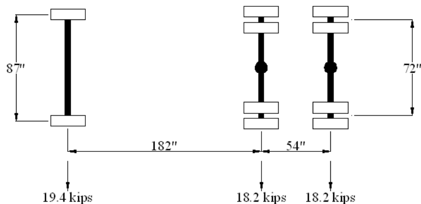
Figure 4.10. Wheel and load configuration for MVRB test vehicle
