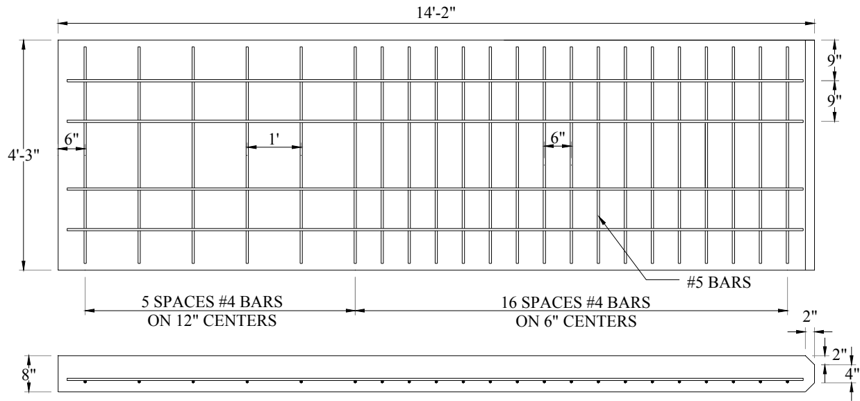
Figure 2.32. Abutment backwall reinforcement details
