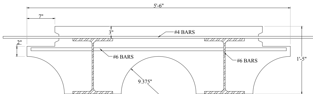
Figure 4.2. Typical cross-section of the PMBISB
