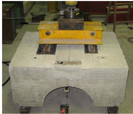
b) Photograph of ultimate load test
