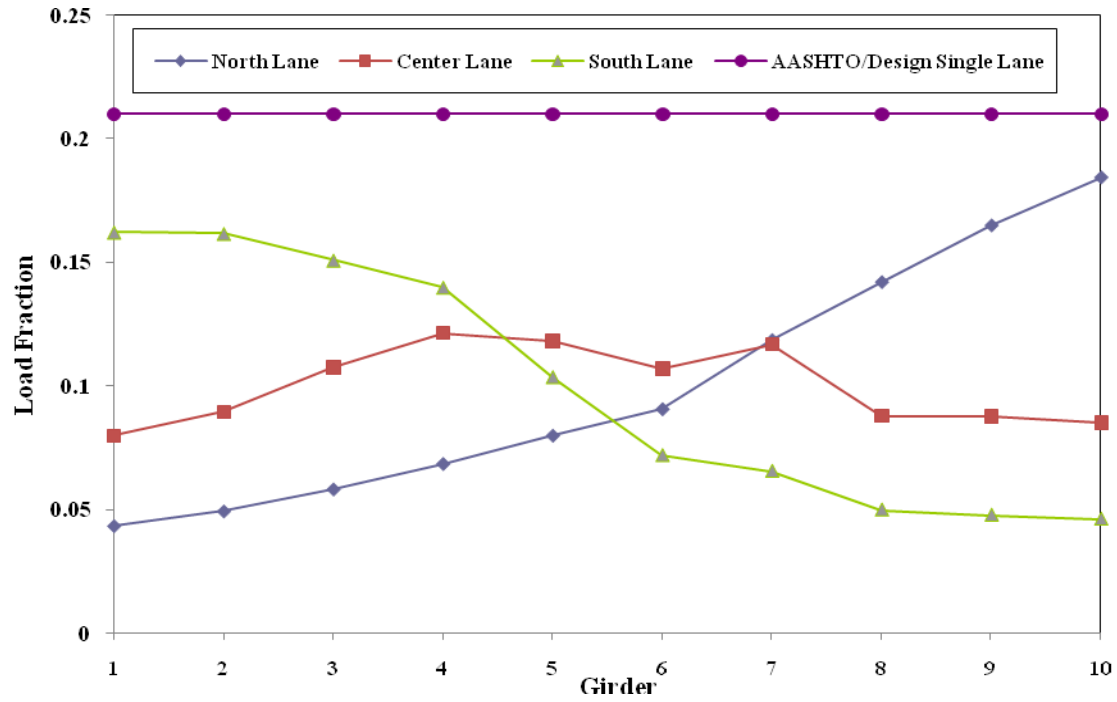
Figure 5.14. Single lane DF from strains
