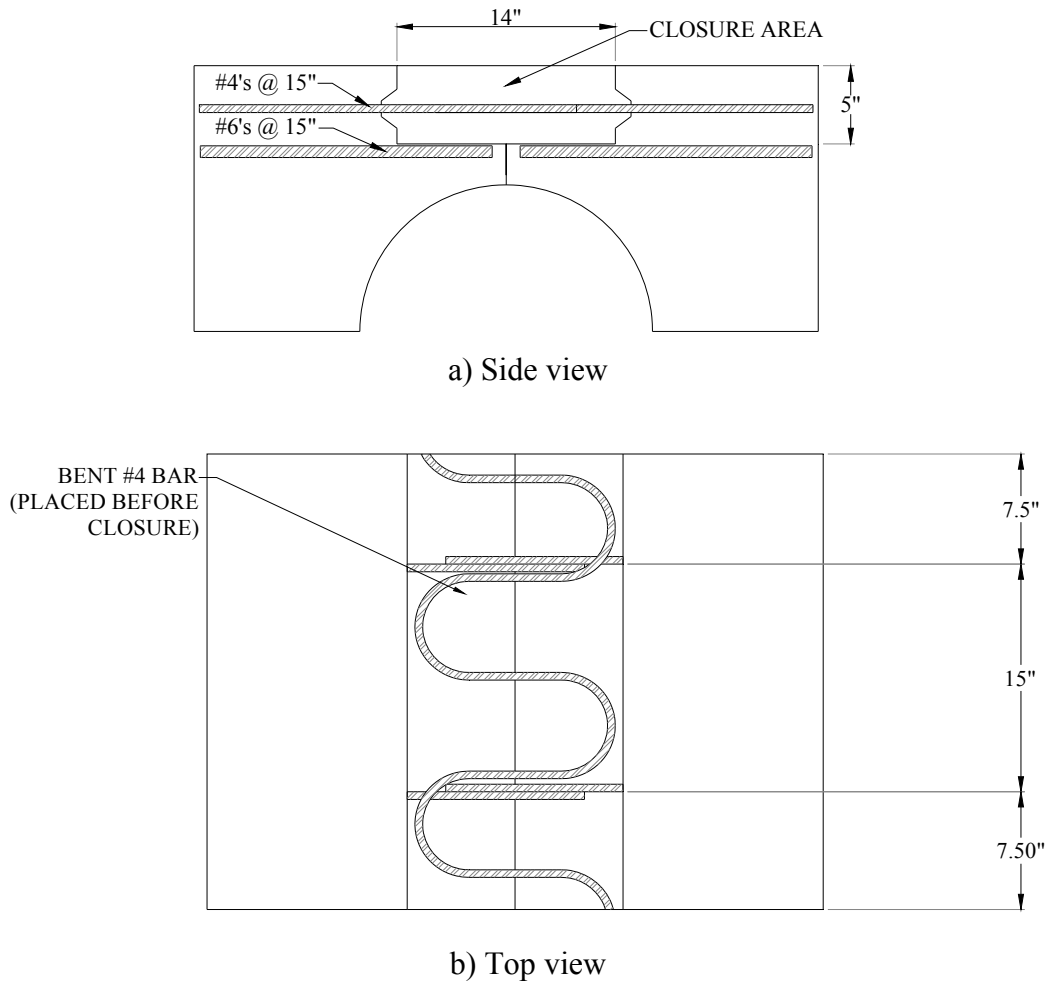
Figure 2.22. Type 3 Connection
