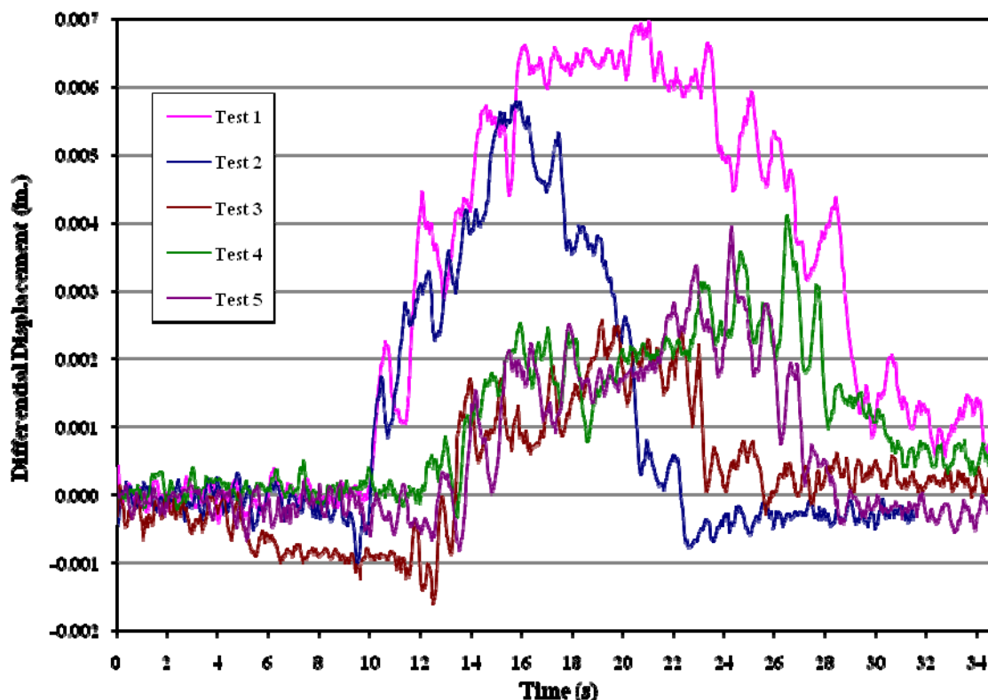
Figure 5.8. Differential displacements along centerline joint
