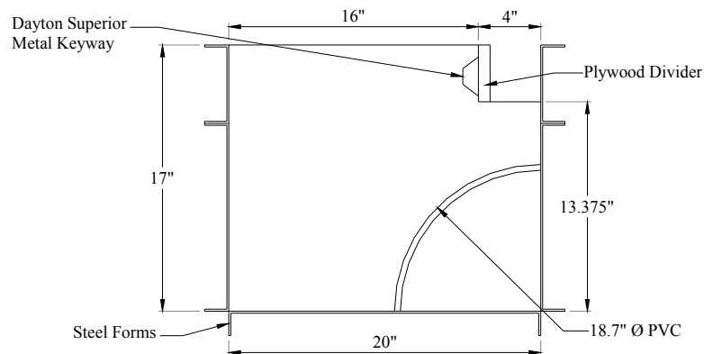
Figure 2.18. Type 2 Connection form details
