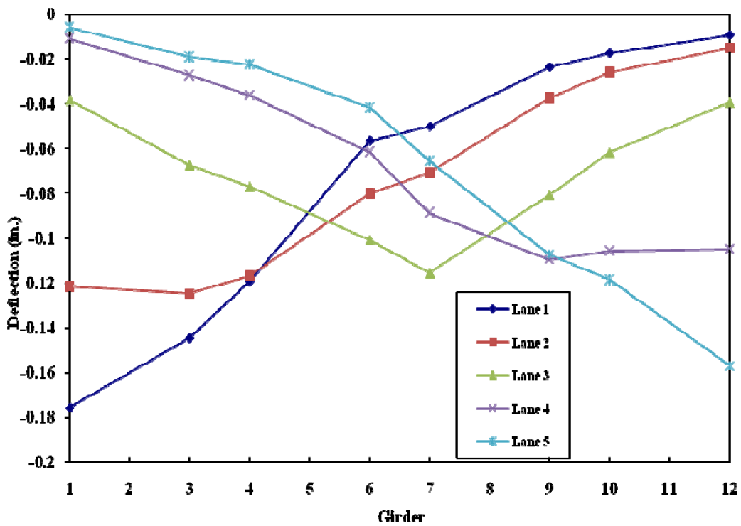
Figure 5.7. Midspan displacement profiles for all five test lanes
