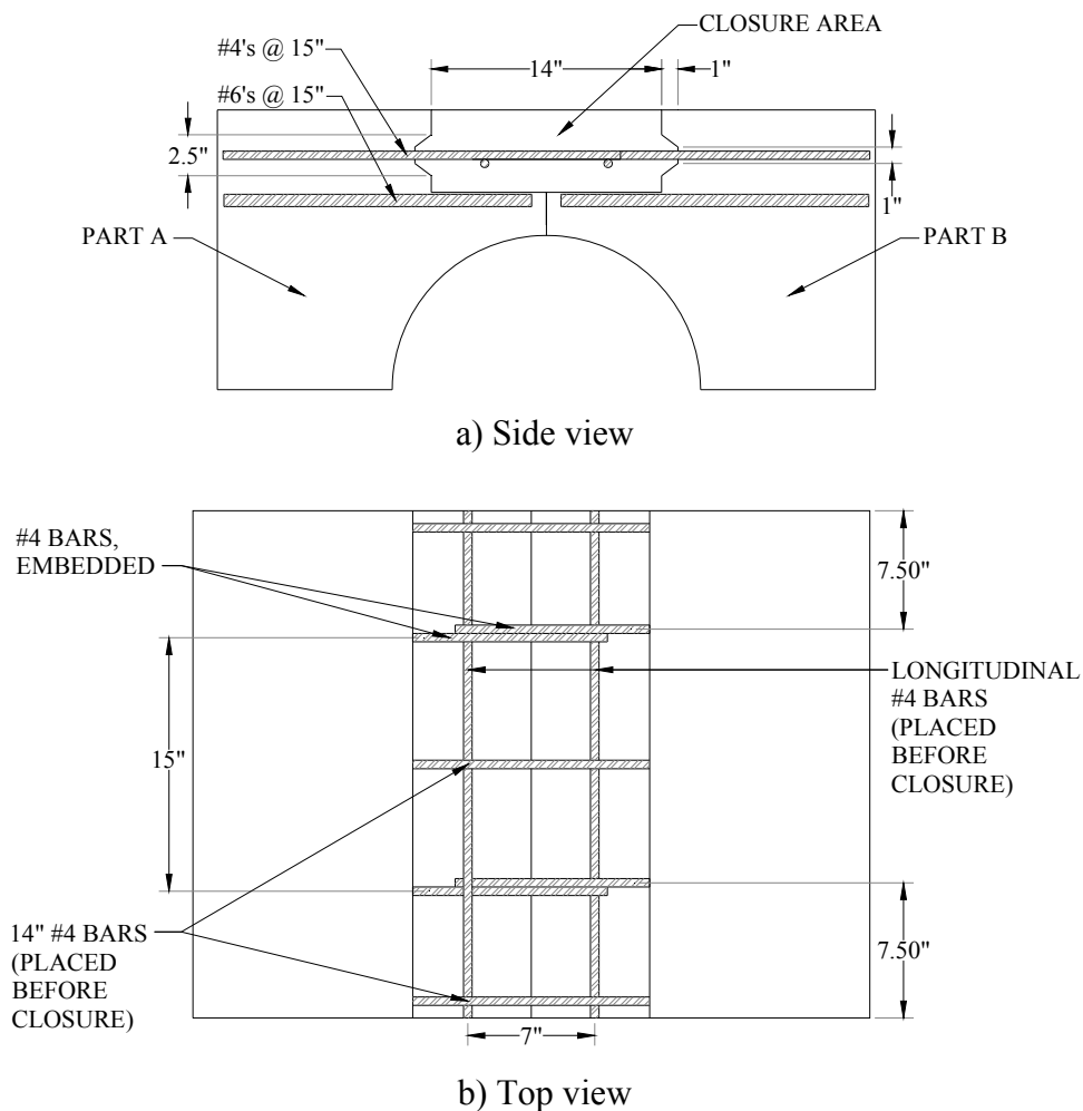
Figure 2.12. Type 1 Connection
