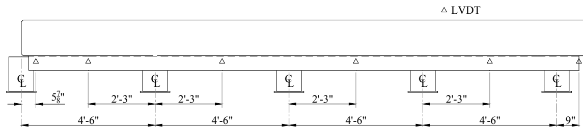
b) Linear variable deflection transducer layout
