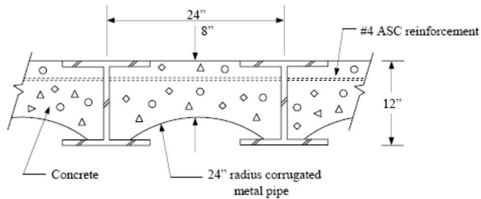
Figure 1.3. MBISB variation 2 cross section
