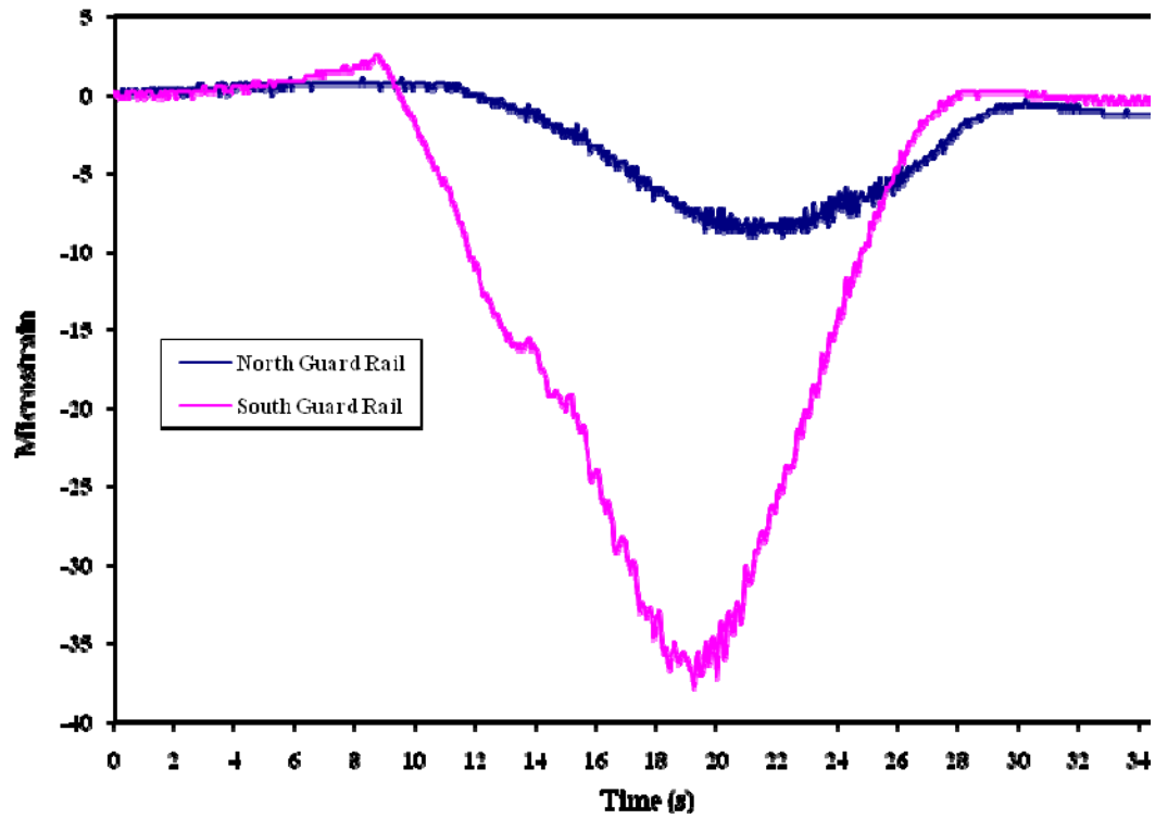
Figure 5.5. Guardrail strains for Test 4.1
