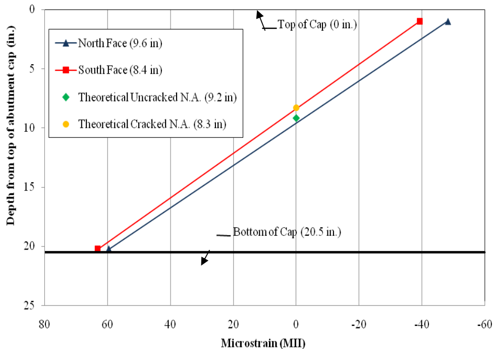
Figure 3.9. Cap 1 neutral axis at Section 2, Load Position 1, 40 kip load
