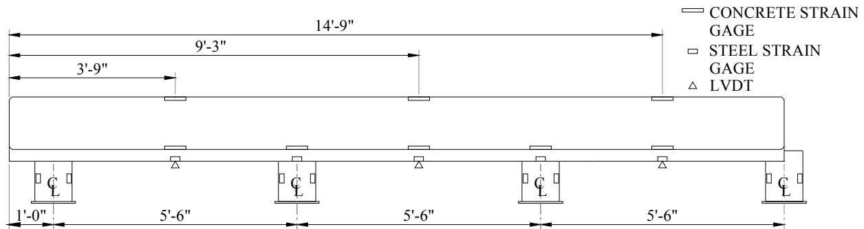
Figure 2.7. Cap 2 instrumentation plan
