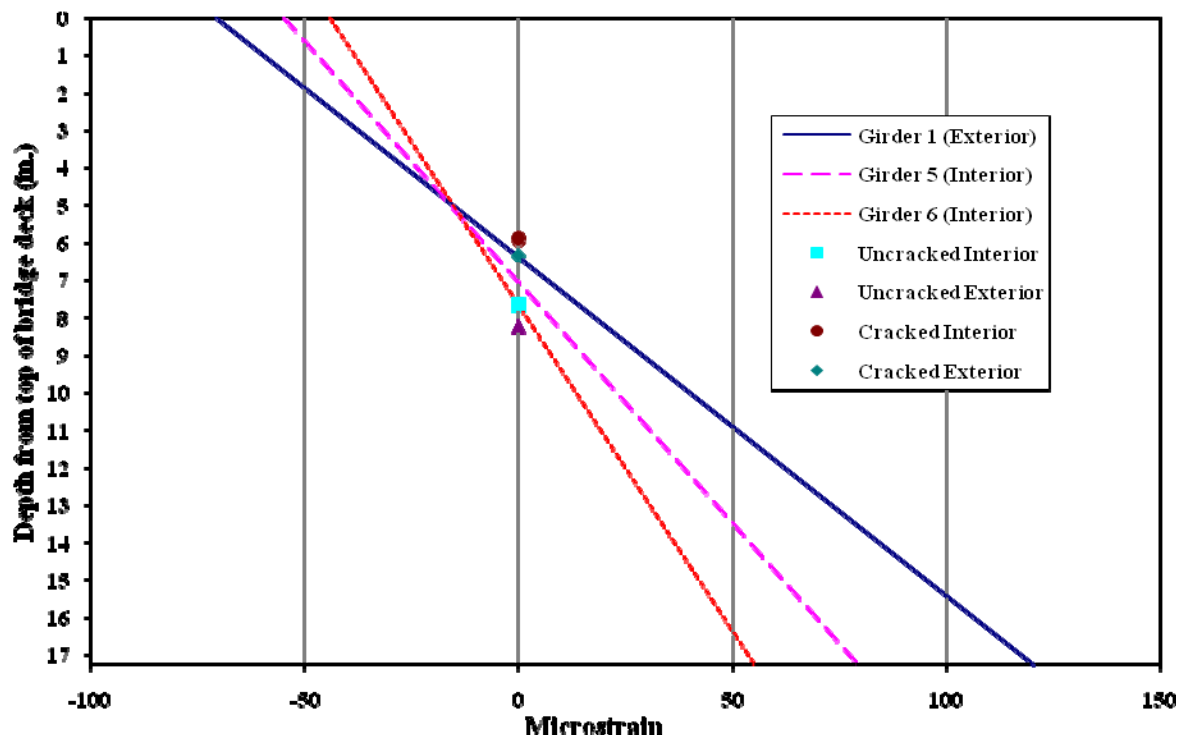
Figure 5.11. Test 3.1 neutral axes
