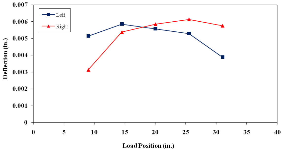
Figure 3.14. Type 1 Connection service deflections
