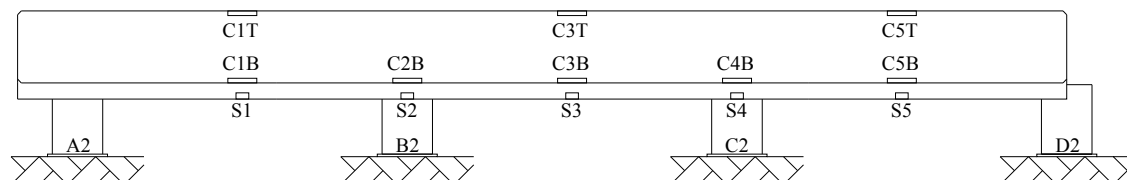
Figure 3.2. Identification of strain gages used on Cap 2
