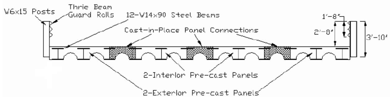
Figure 1.4. PMBISB cross section
