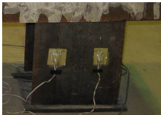
c) Strain gages on pile section in laboratory
