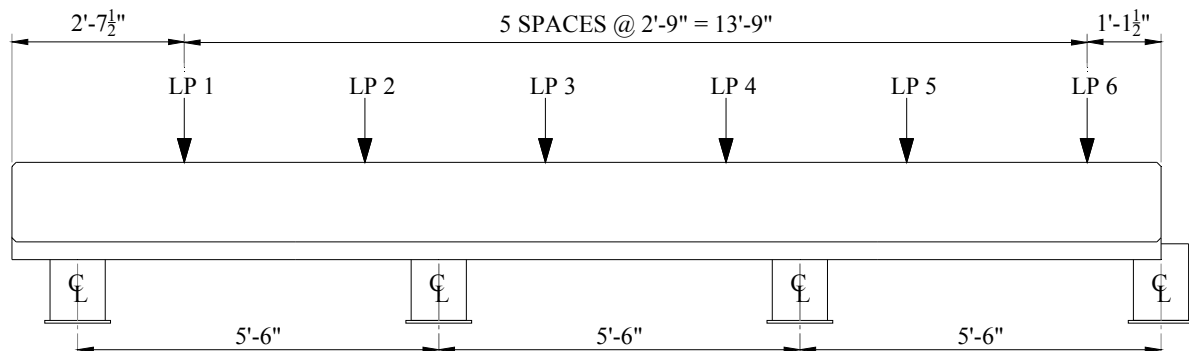
Figure 2.8. Cap 2 service test set-up
