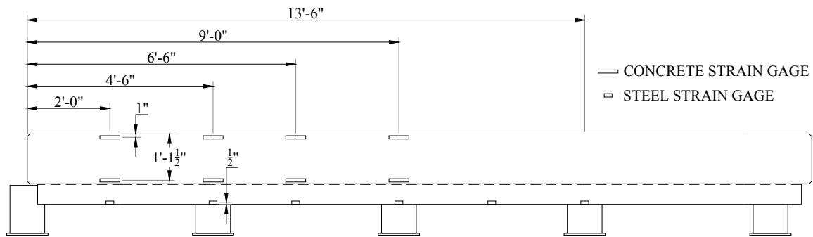
a) Strain gage layout
