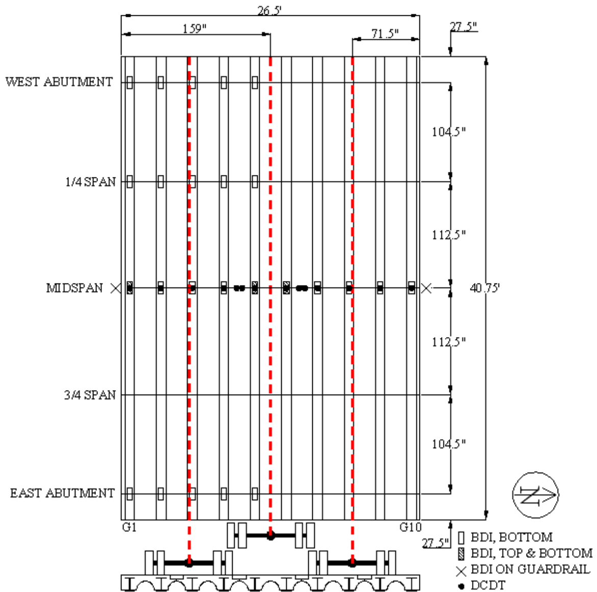
Figure 4.18. Instrumentation and loading lane layout for MRB
