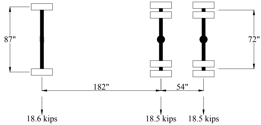
Figure 4.17. Wheel and load configuration for MRB test vehicle
