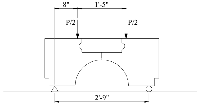
a) Ultimate load points
