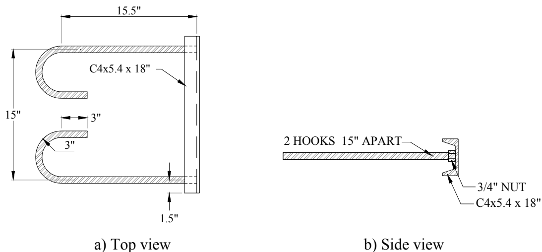
Figure 2.19. Type 2 Connection reinforcing detail
