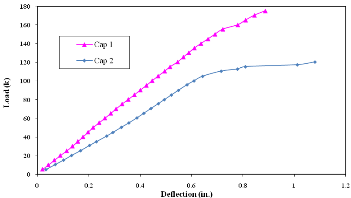
Figure 3.12. Plot of load vs. deflection for positive capacity tests of caps
