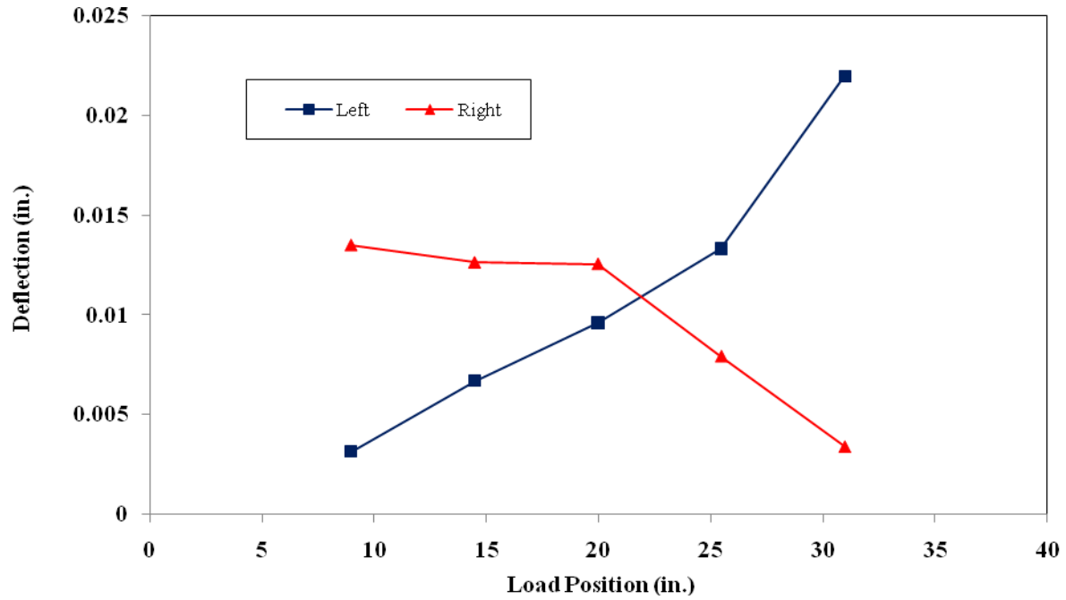
Figure 3.16. Type 3 Connection service deflections
