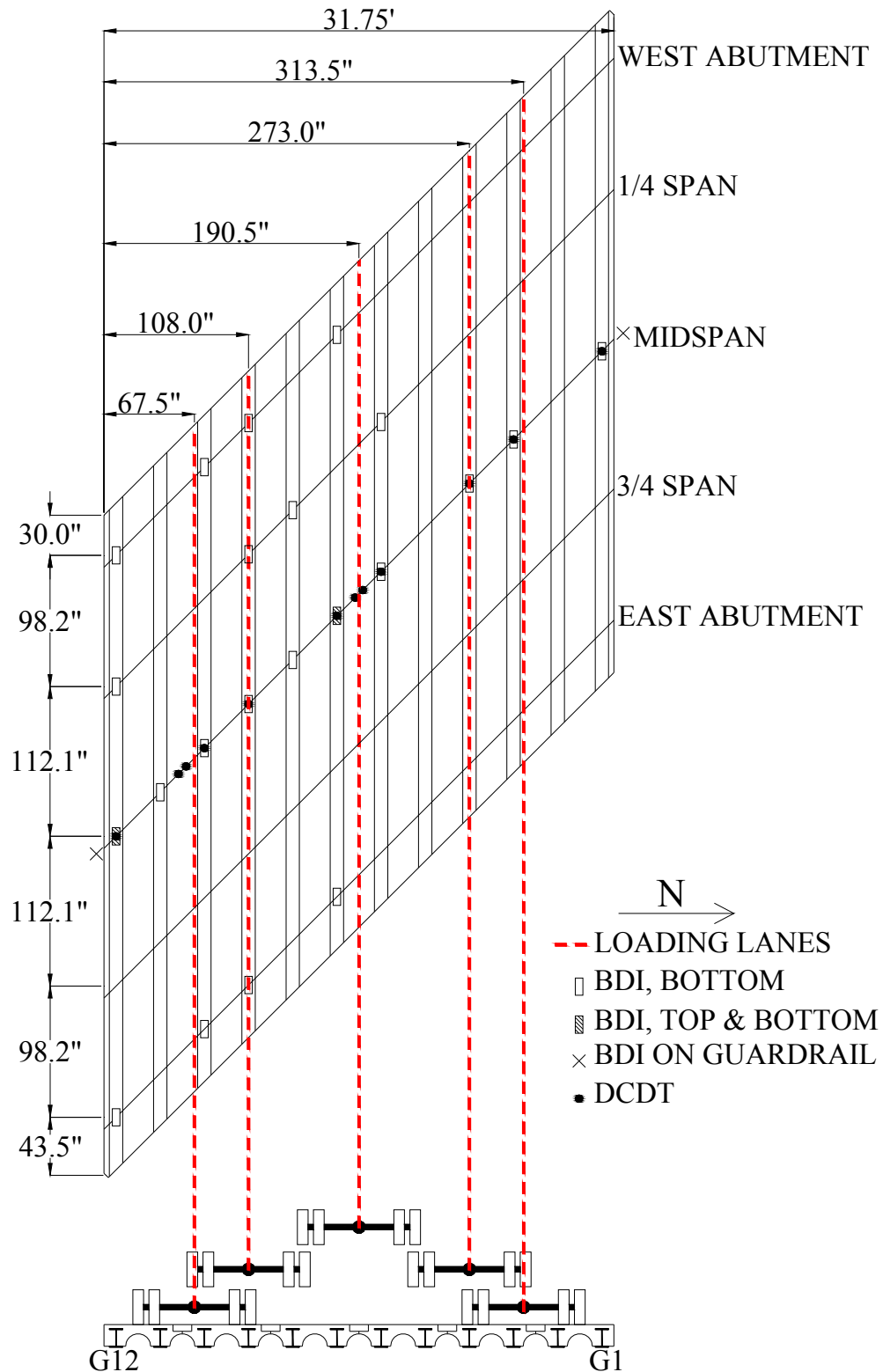
Figure 4.11. Instrumentation and loading lane layout for MVRB
