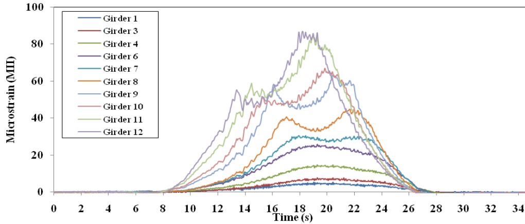
Figure 5.2. Midspan strain history for Test 5.1
