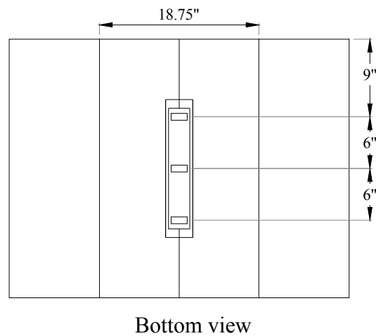
Figure 2.29. Additional strain gages positioned on bottom plate in Type 2 Connections
