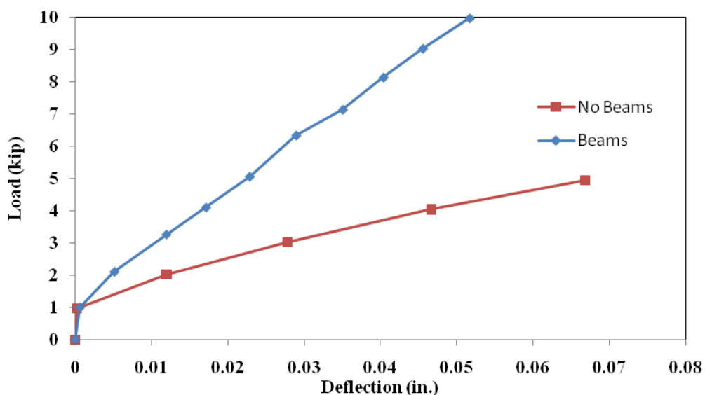
Figure 3.19. Load-deflection curves for Load Point 2 at LVDT DC2
