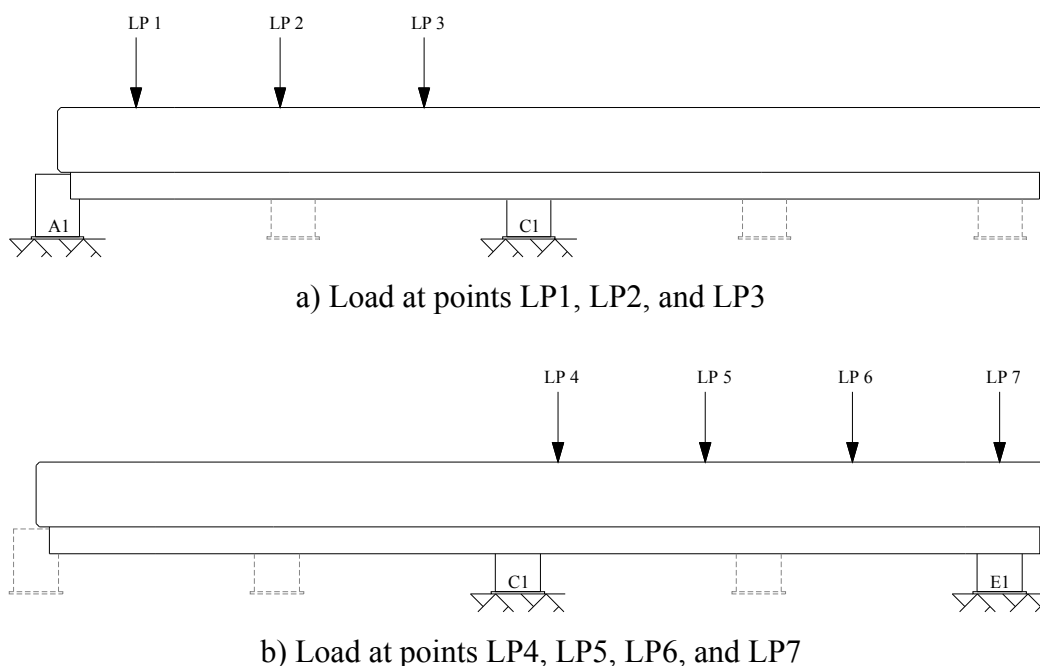
Figure 3.3. Support conditions for Cap 1 for each load point.
