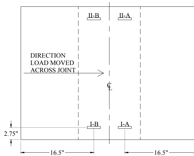
Figure 3.17. Labeling for top concrete strain gages
