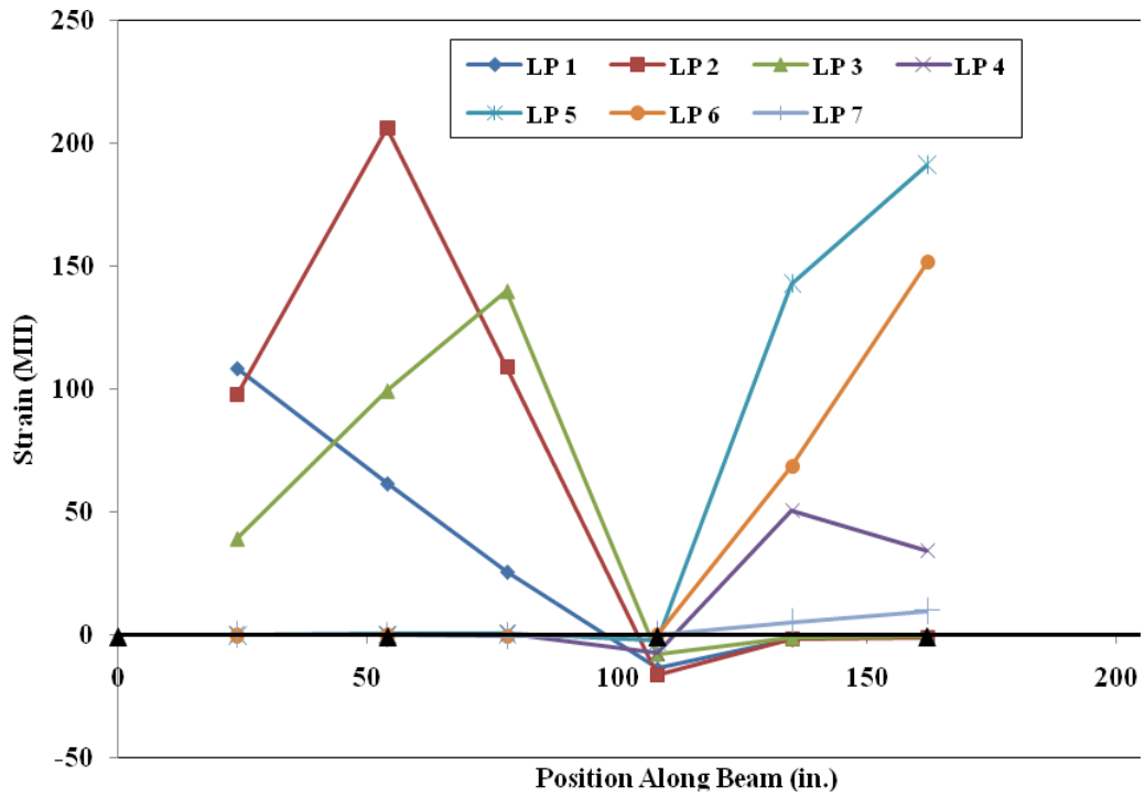
Figure 3.7. Steel strains for Cap 1 for the seven load points used
