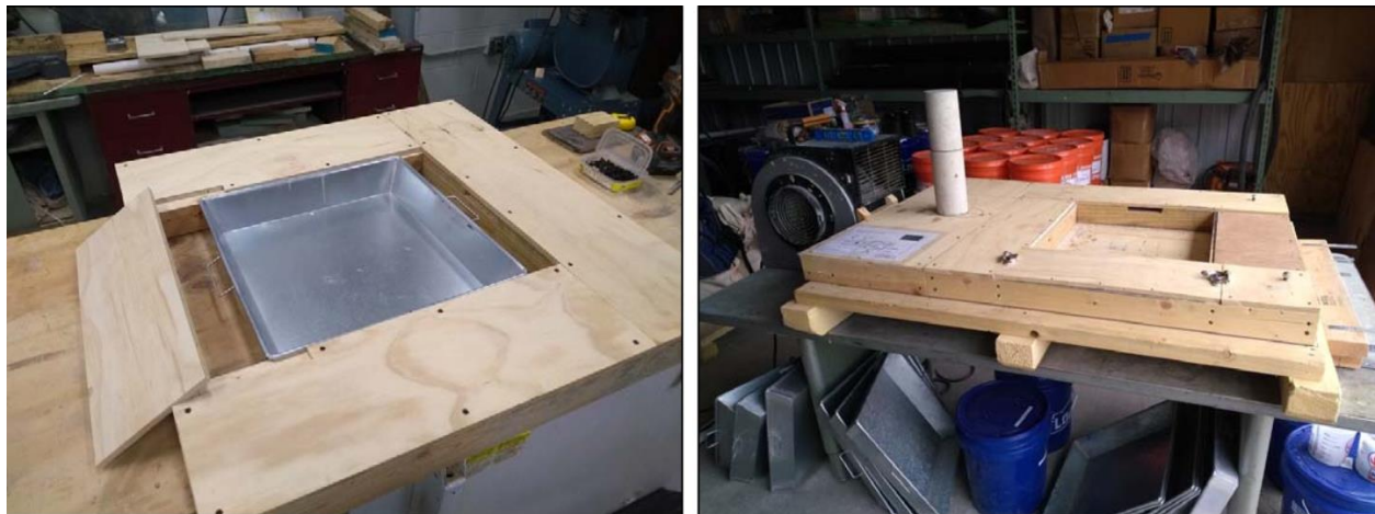
Figure 34. Wind erosion test apparatus during fabrication and final construction
