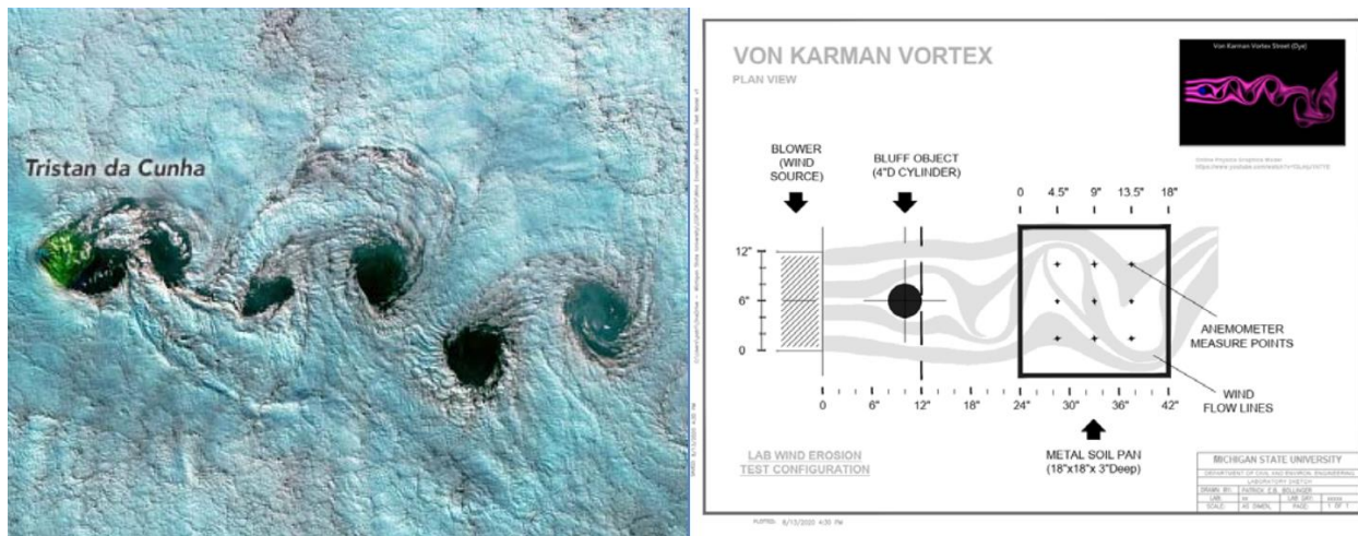
Figure 35. Von Karman Vortex Street (left) and AutoCAD-scaled version for WETA layout (right)
