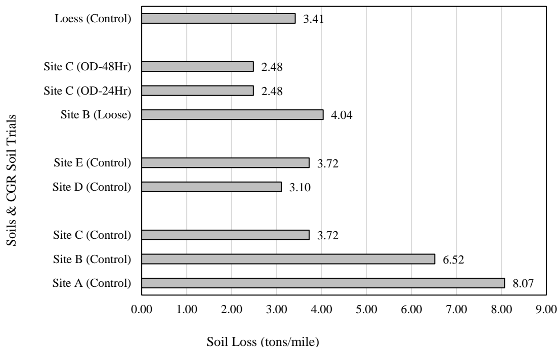
Figure 45. Wind erosion soil loss results for untreated soils
