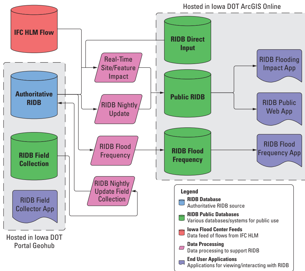
Overview of systems architecture for RIDB
